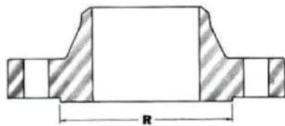
Raised-Face
