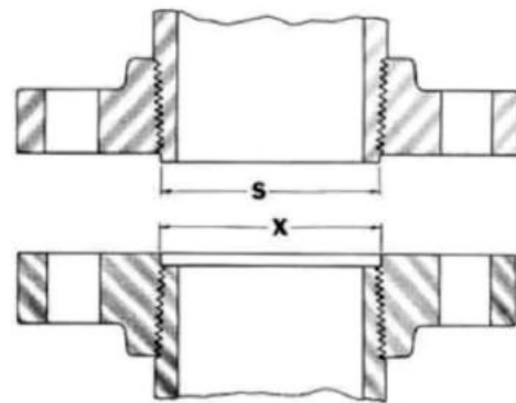
Small-Male-and-Female on-end-of-pipe
