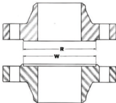
Large-Male-and-Female
